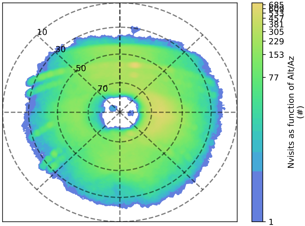
too_combined_no_nss_s10.0_v3.4_10yrs u: Nvisits as function of Alt/Az
