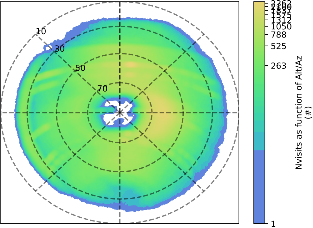
too_combined_no_nss_s10.0_v3.4_10yrs r: Nvisits as function of Alt/Az
