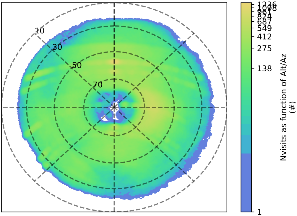
too_combined_no_nss_s10.0_v3.4_10yrs g: Nvisits as function of Alt/Az
