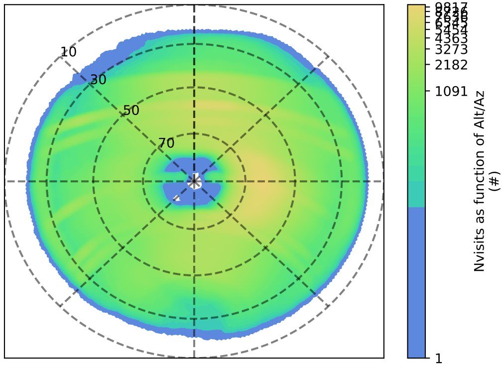
too_combined_no_nss_s10.0_v3.4_10yrs : Nvisits as function of Alt/Az
