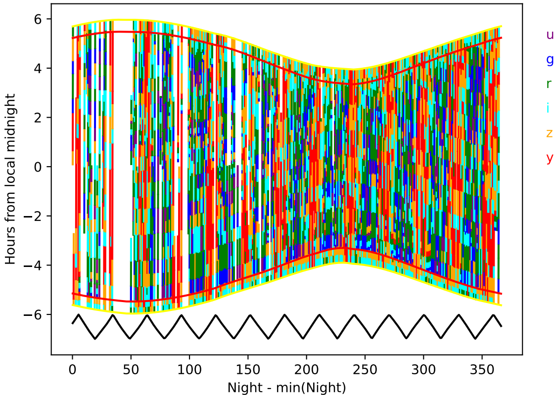
too_combined_no_nss_s10.0_v3.4_10yrs year 6-7: Hourglass
