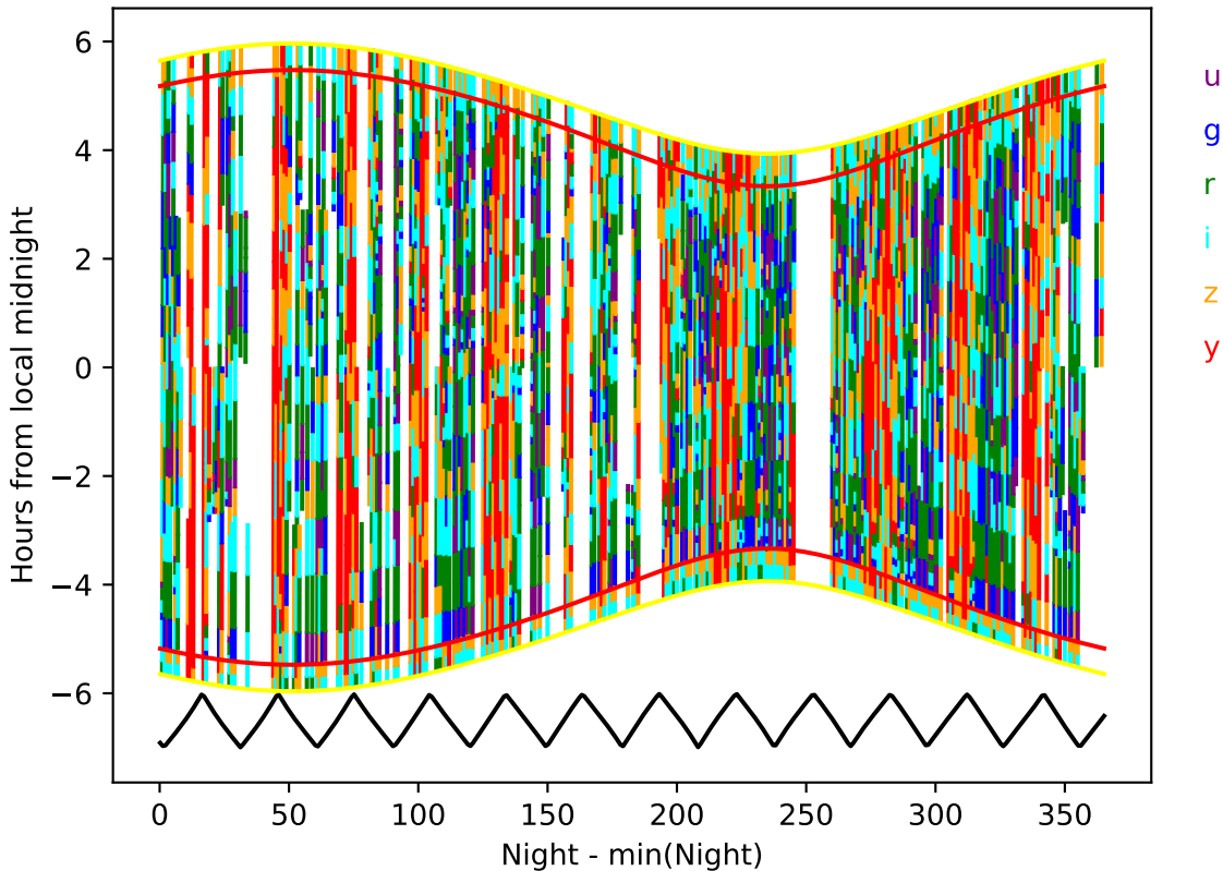
too_combined_no_nss_s10.0_v3.4_10yrs year 5-6: Hourglass
