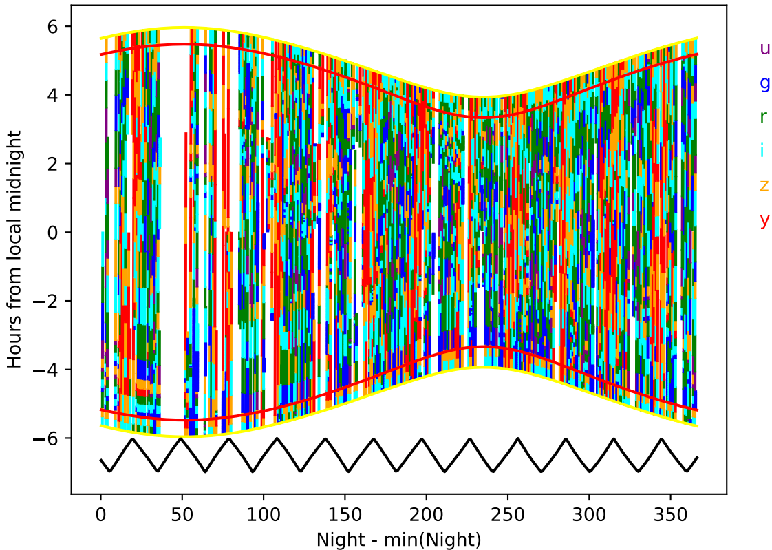
too_combined_no_nss_s10.0_v3.4_10yrs year 2-3: Hourglass
