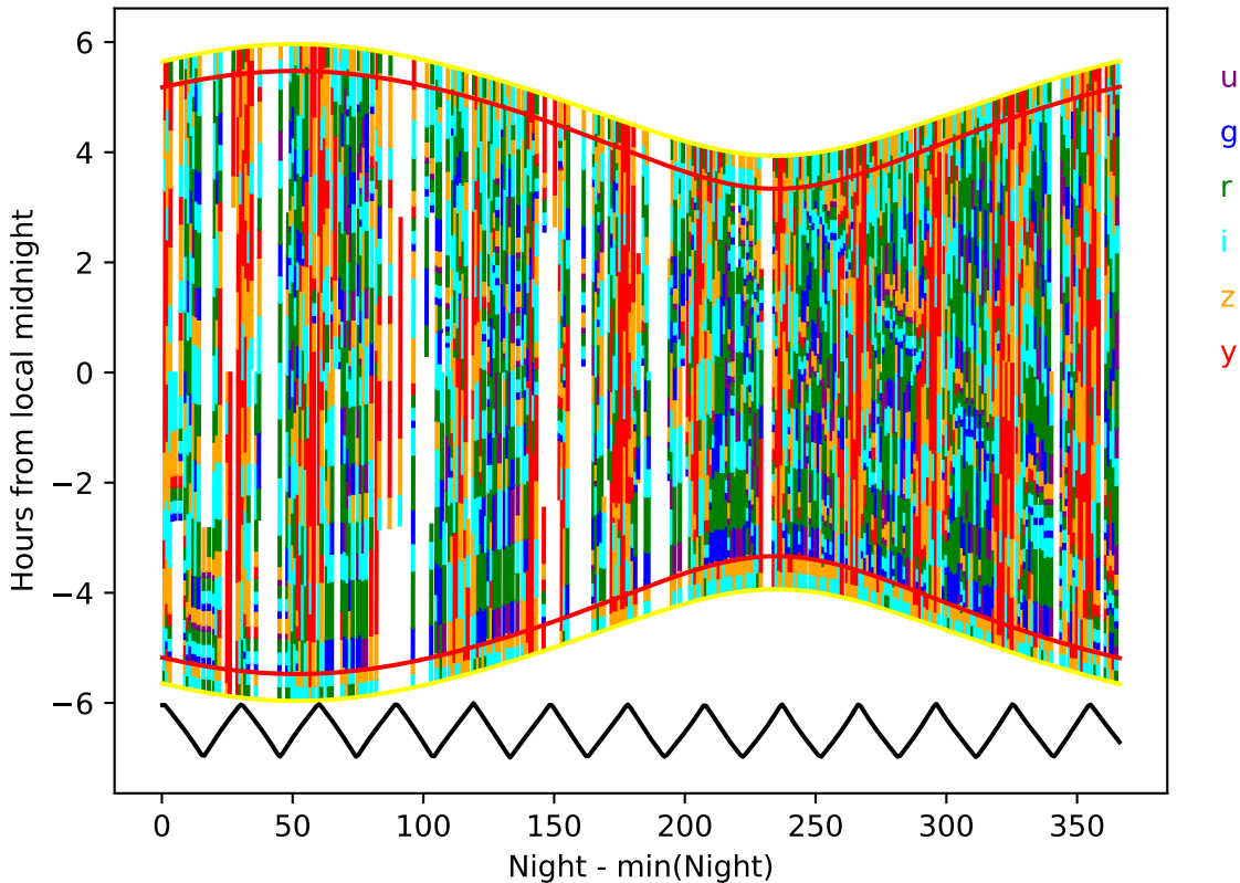
too_combined_no_nss_s10.0_v3.4_10yrs year 1-2: Hourglass
