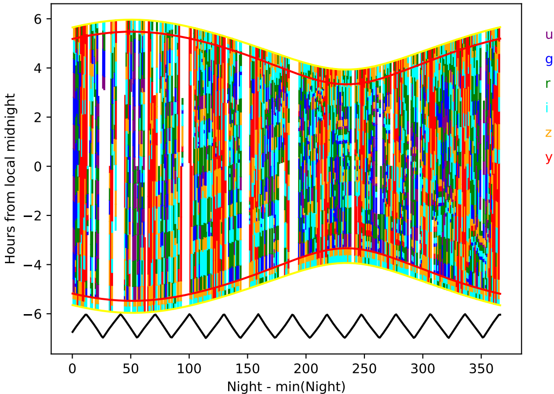
too_combined_no_nss_s10.0_v3.4_10yrs year 0-1: Hourglass
