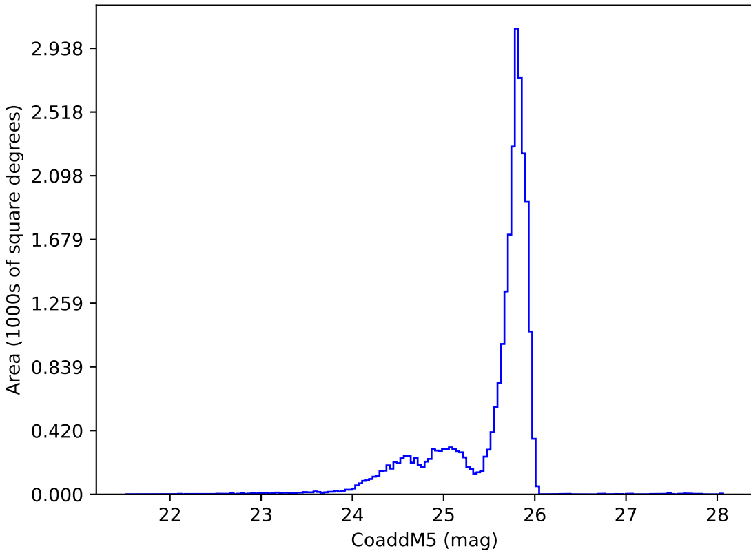
too_combined_no_nss_s10.0_v3.4_10yrs z: CoaddM5
