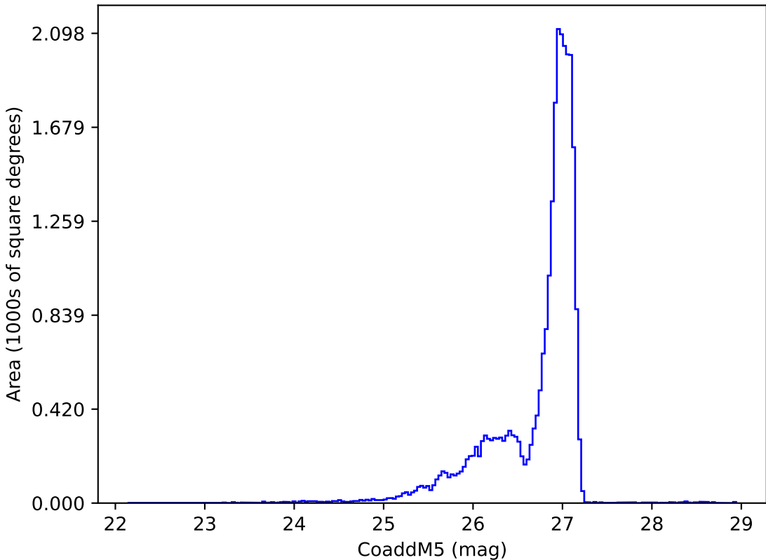
too_combined_no_nss_s10.0_v3.4_10yrs r: CoaddM5
