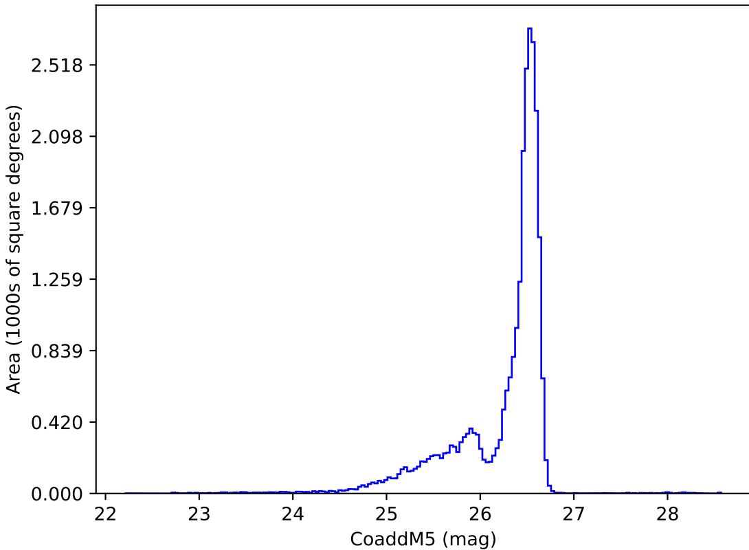
too_combined_no_nss_s10.0_v3.4_10yrs i: CoaddM5
