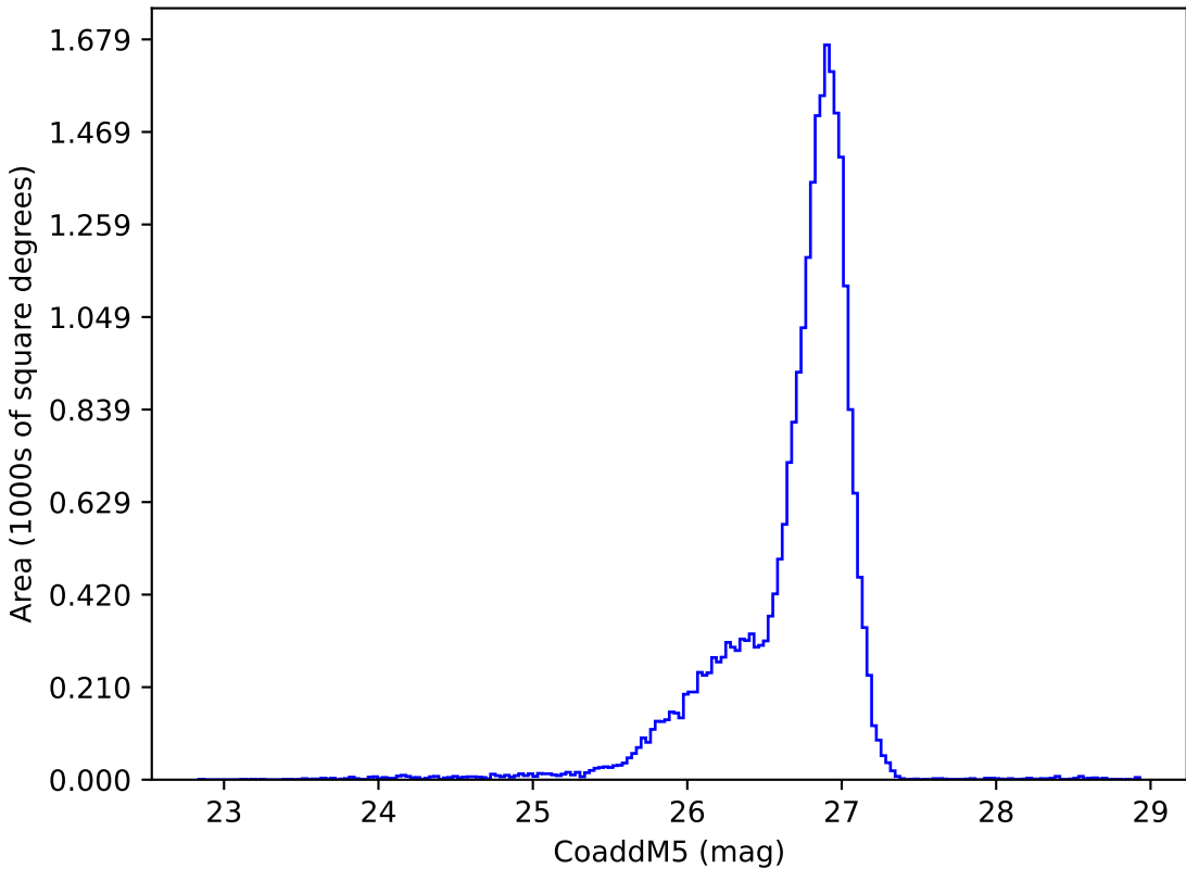
too_combined_no_nss_s10.0_v3.4_10yrs g: CoaddM5
