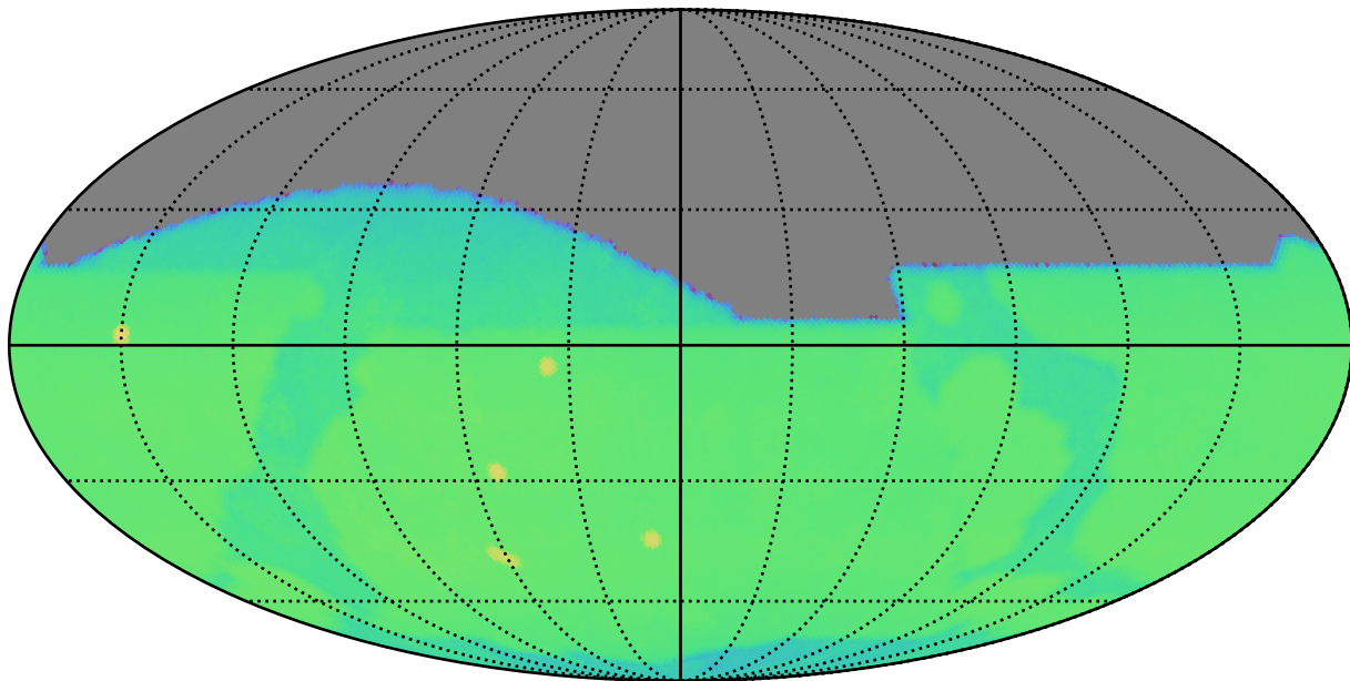
too_combined_no_nss_s10.0_v3.4_10yrs : CoaddM5
