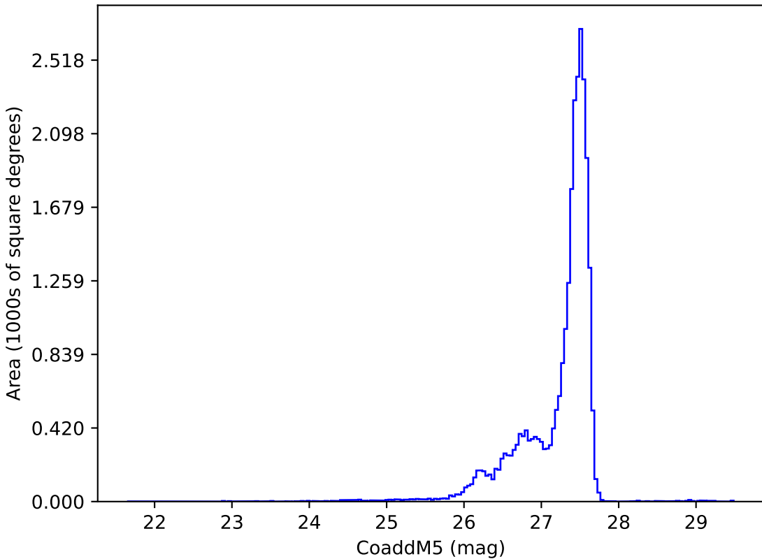
too_combined_no_nss_s10.0_v3.4_10yrs : CoaddM5
