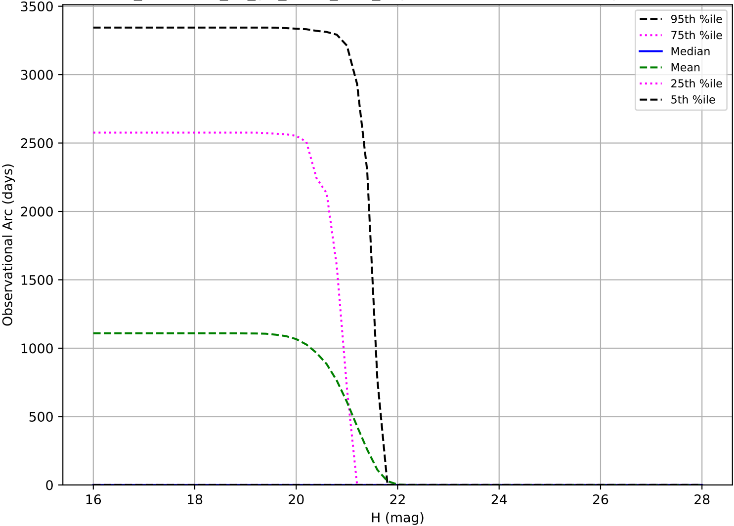
too_combined_no_gw_s10.0_v3.4_10yrs: Observational Arc Length Vatira
