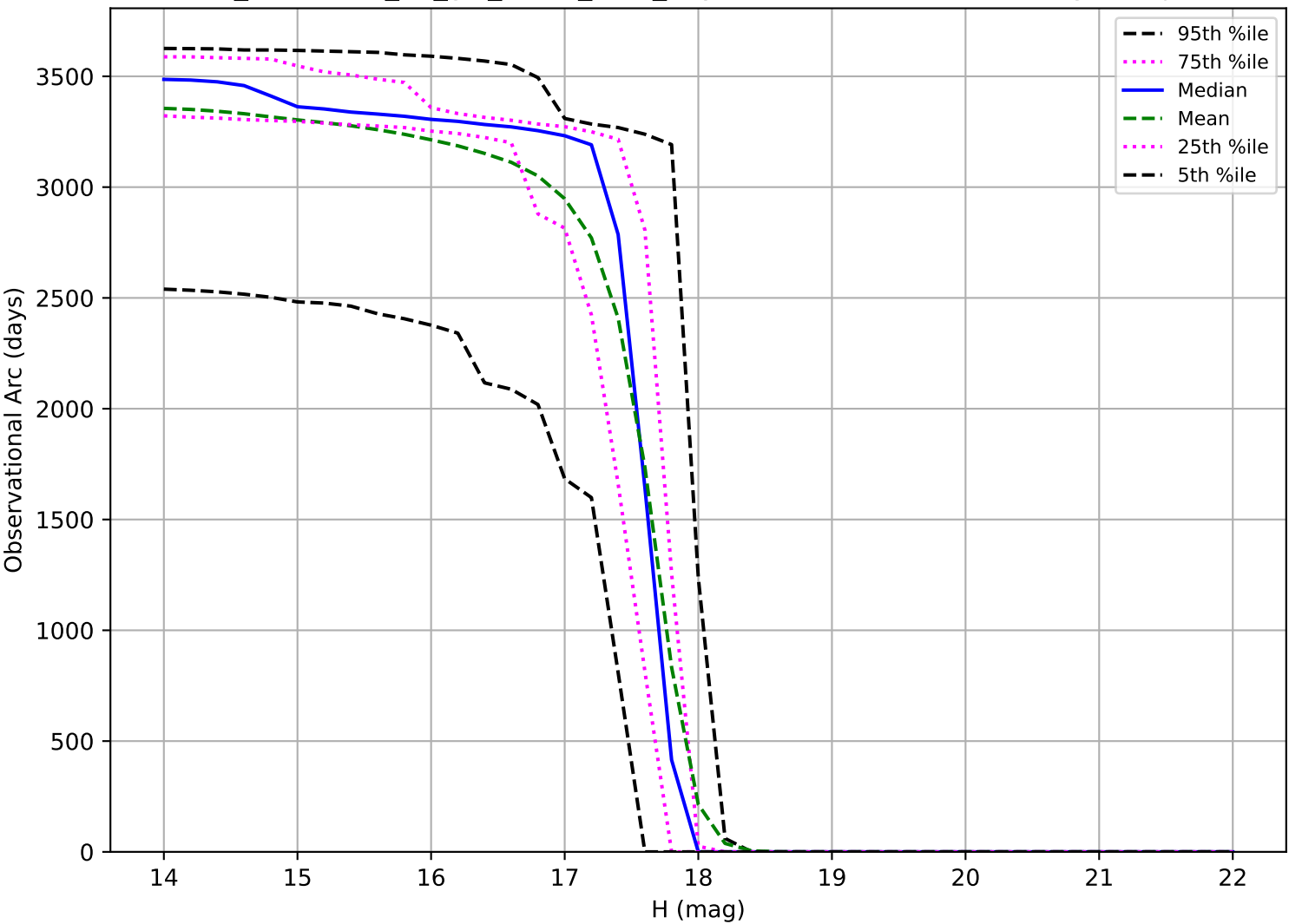
too_combined_no_gw_s10.0_v3.4_10yrs: Observational Arc Length Trojan
