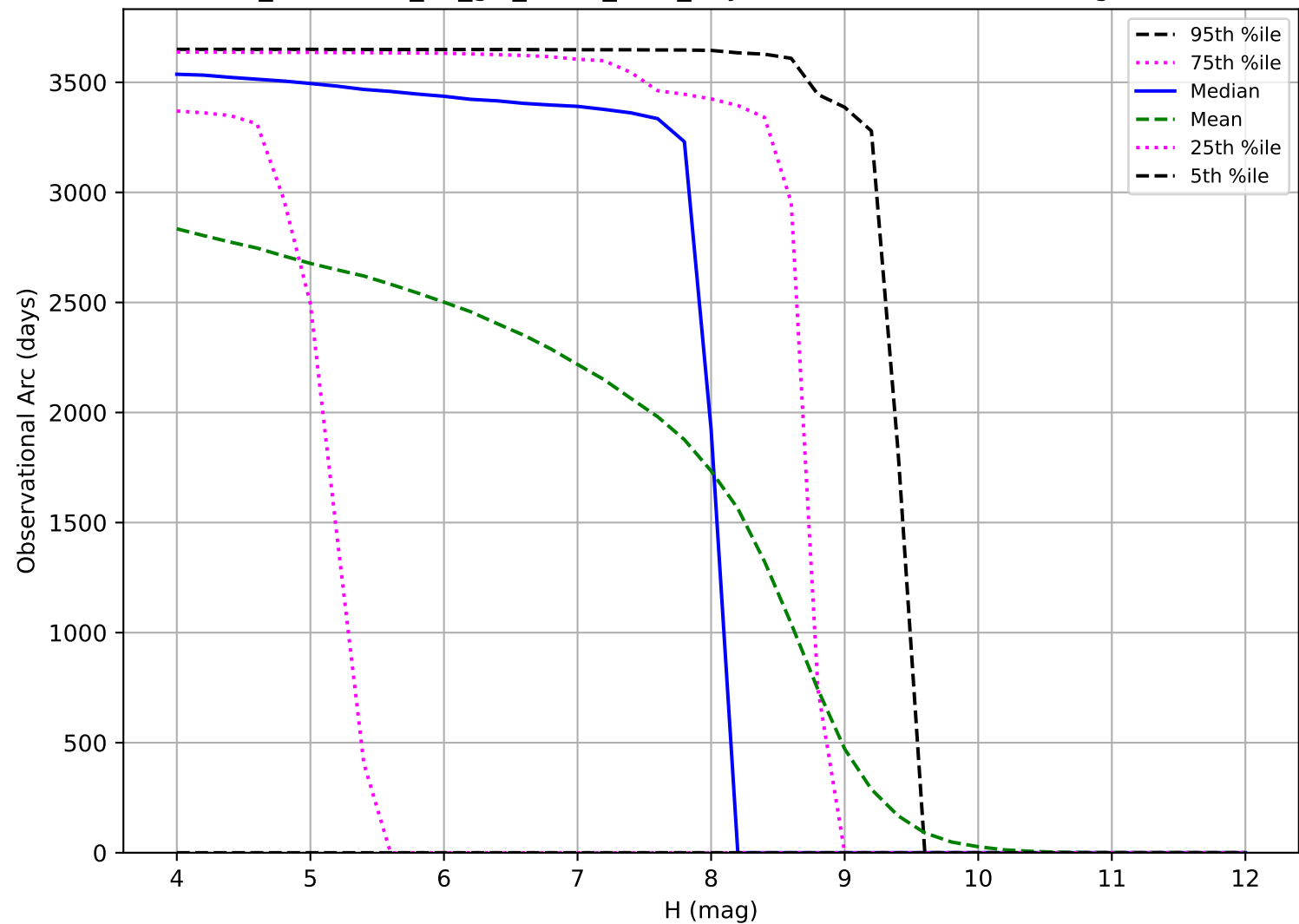
too_combined_no_gw_s10.0_v3.4_10yrs: Observational Arc Length TNO
