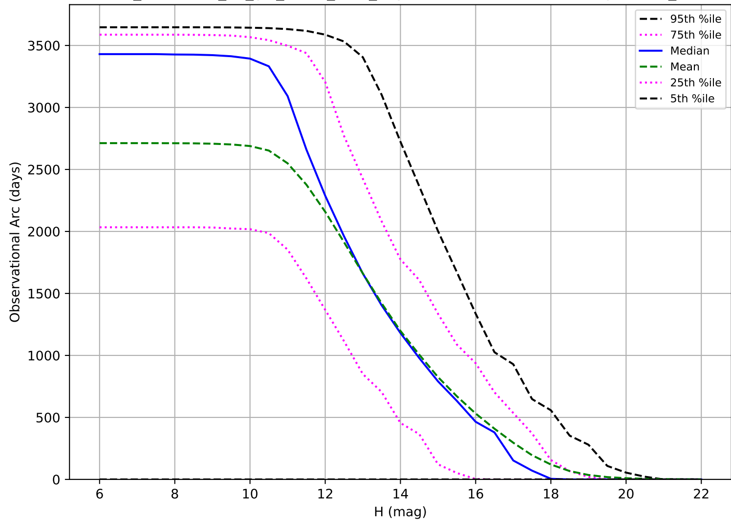
too_combined_no_gw_s10.0_v3.4_10yrs: Observational Arc Length OCC_r5
