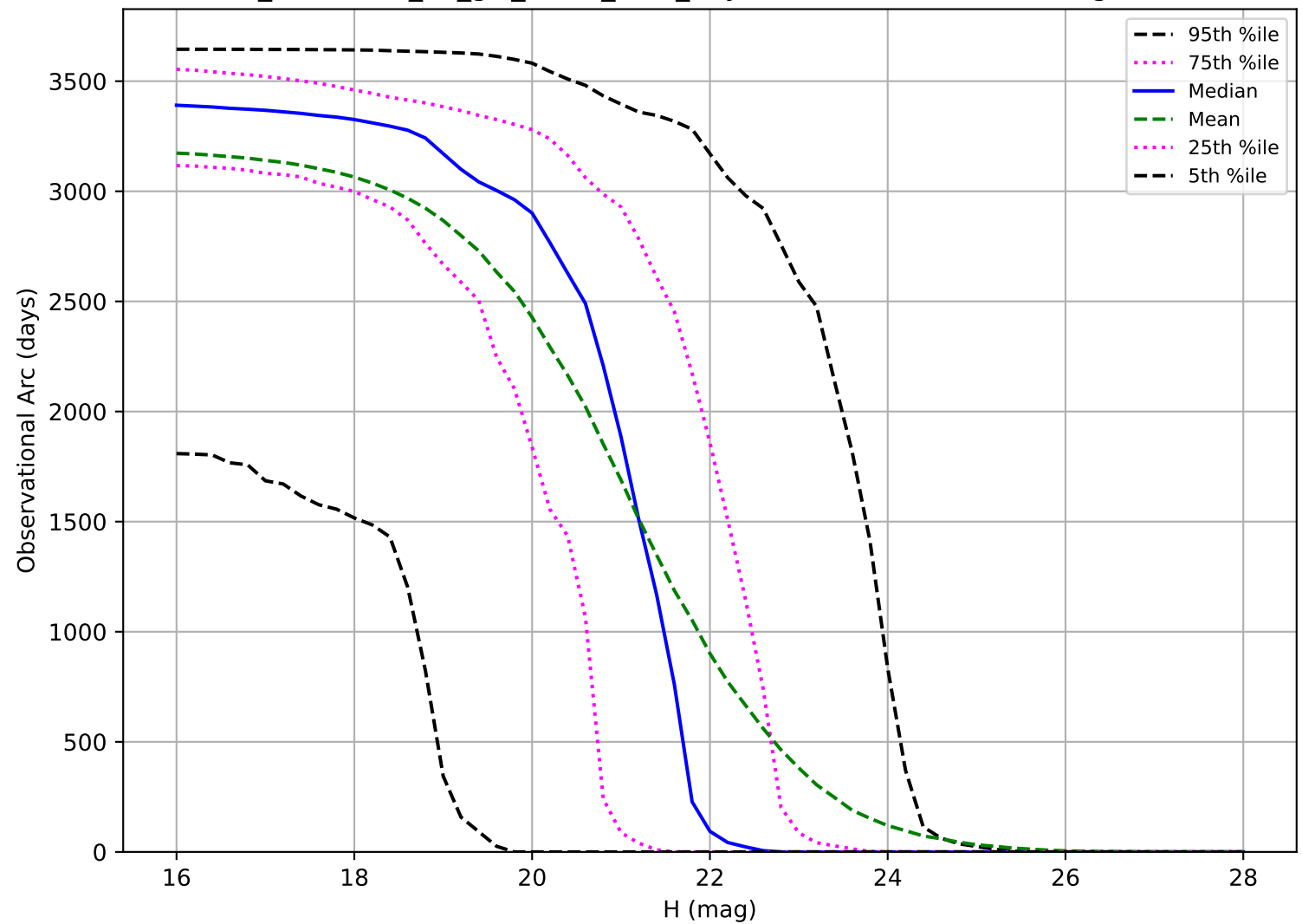
too_combined_no_gw_s10.0_v3.4_10yrs: Observational Arc Length NEO
