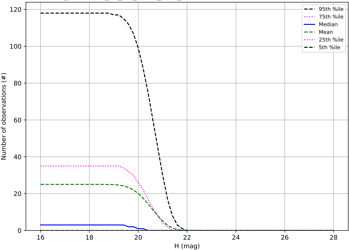
too_combined_no_gw_s10.0_v3.4_10yrs: Number of observations Vatira
