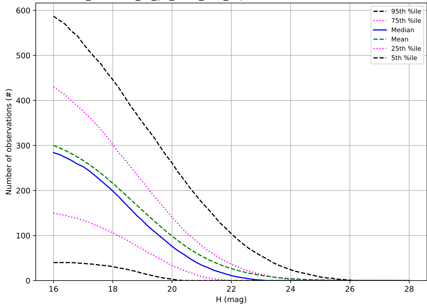
too_combined_no_gw_s10.0_v3.4_10yrs: Number of observations PHA
