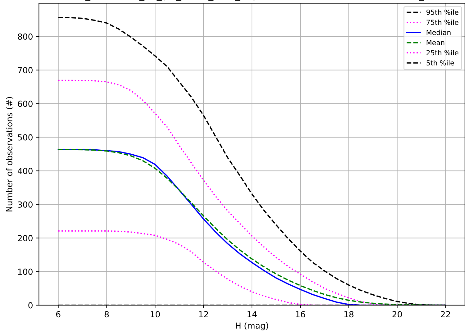
too_combined_no_gw_s10.0_v3.4_10yrs: Number of observations OCC_r5
