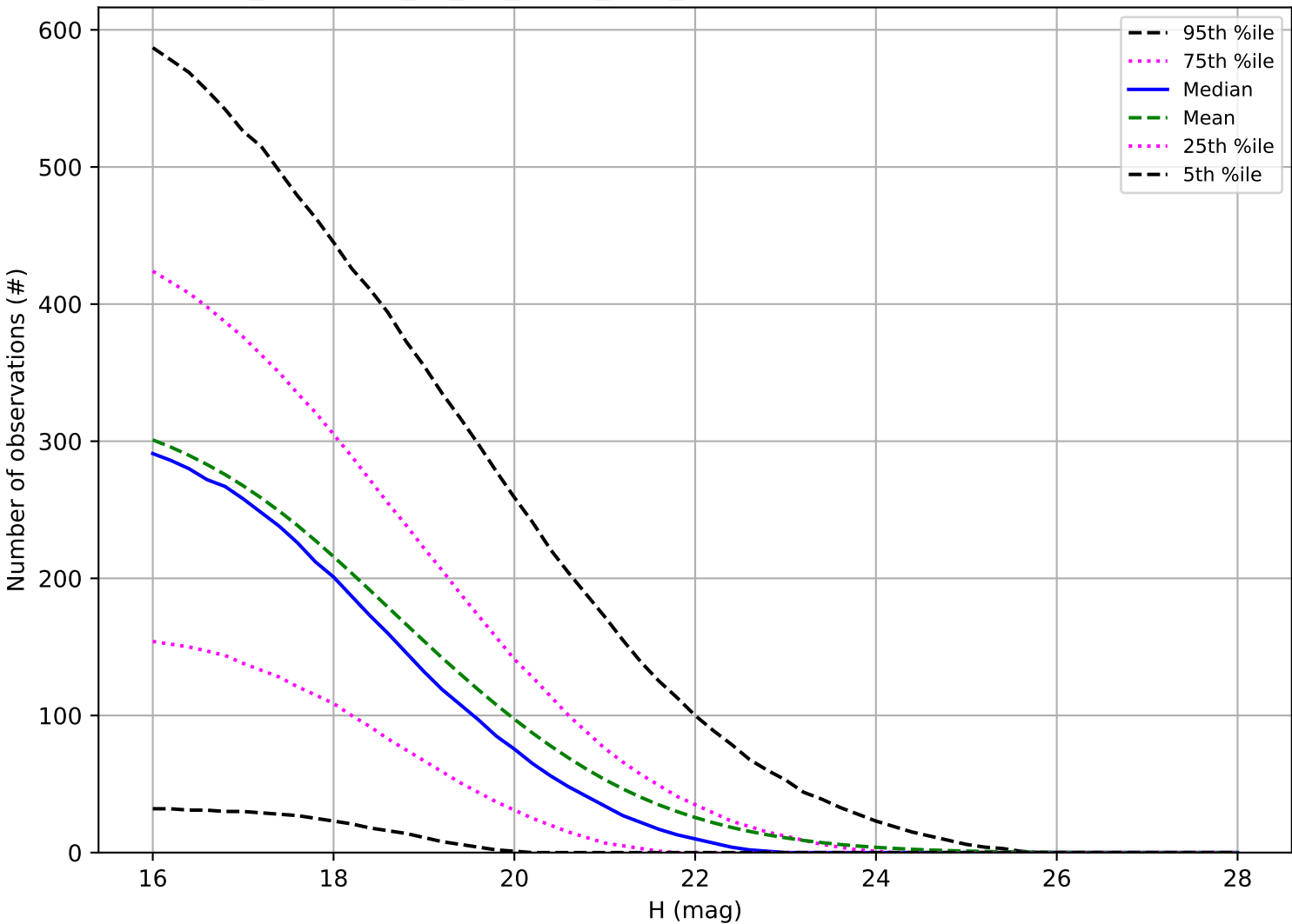
too_combined_no_gw_s10.0_v3.4_10yrs: Number of observations NEO
