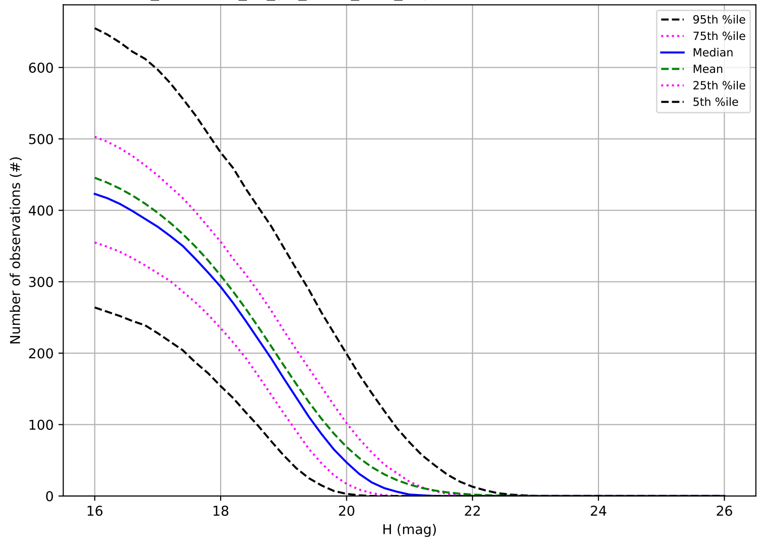
too_combined_no_gw_s10.0_v3.4_10yrs: Number of observations MBA
