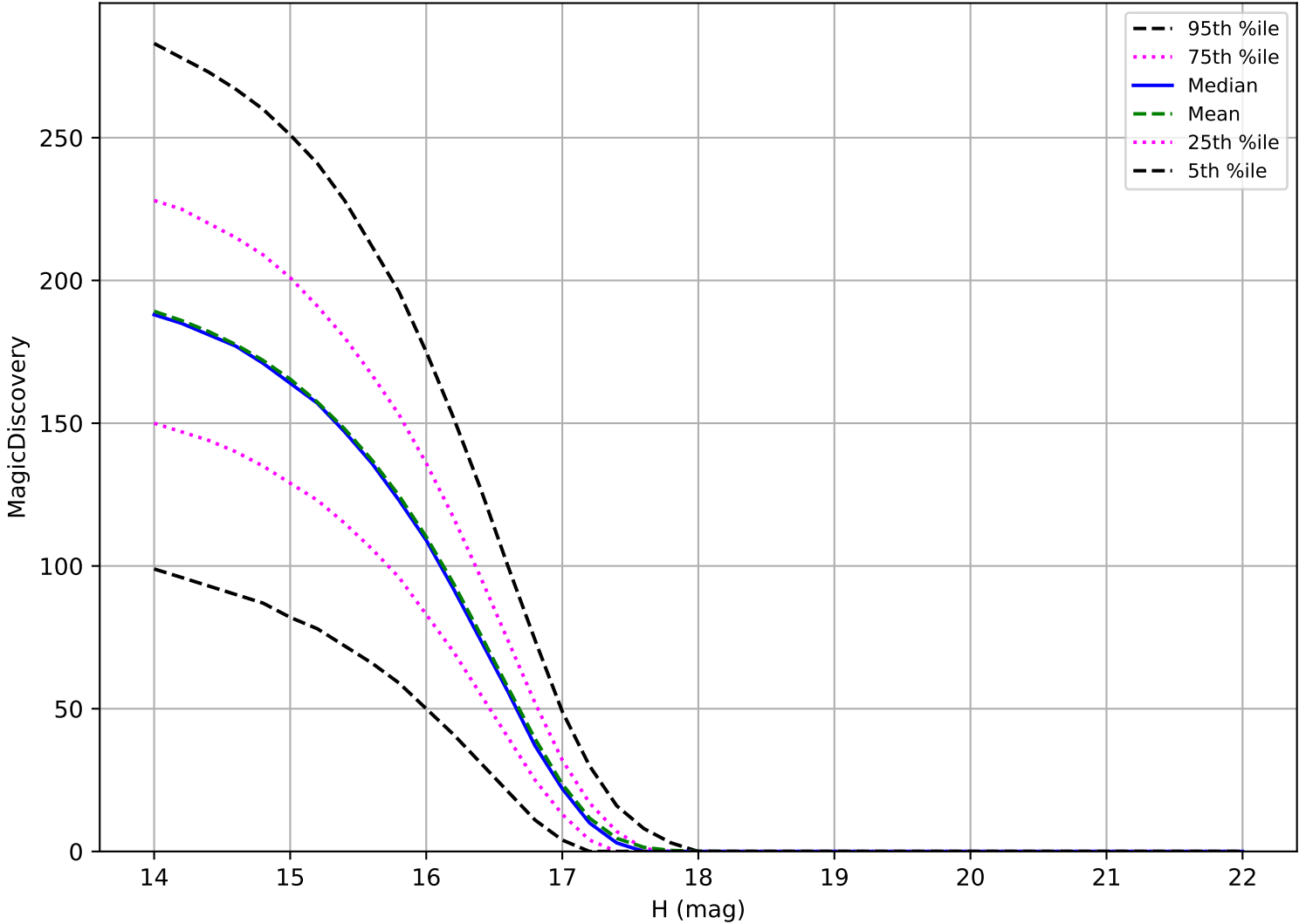
too_combined_no_gw_s10.0_v3.4_10yrs: Trojan 6 detections in 60 nights detection loss
