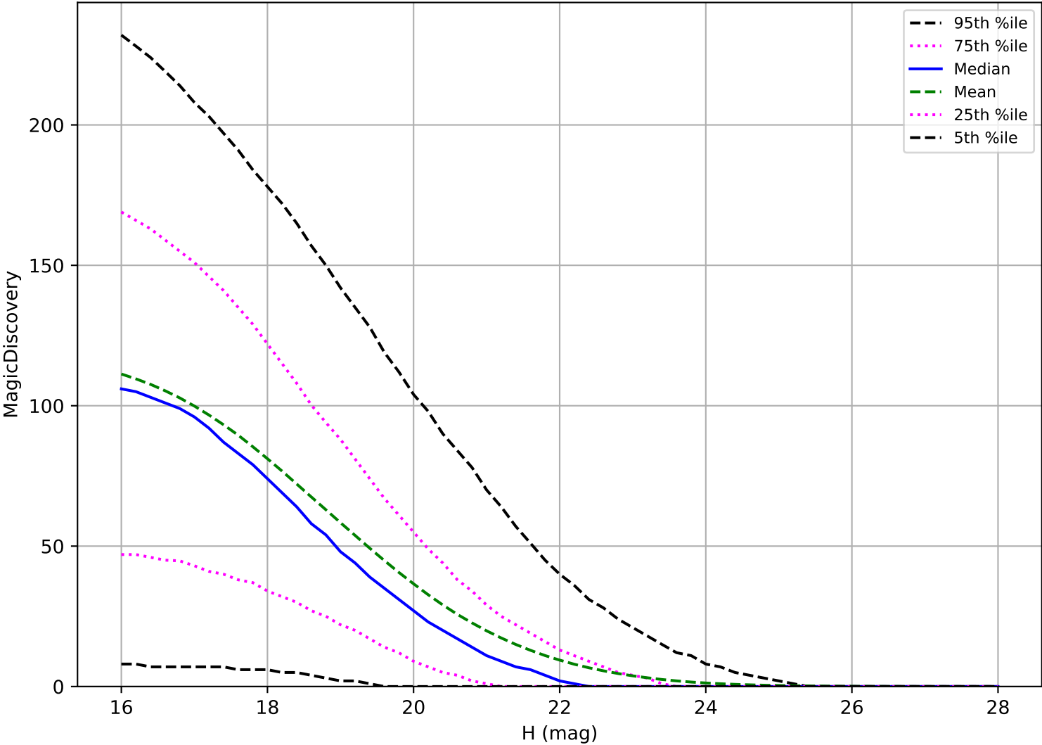
too_combined_no_gw_s10.0_v3.4_10yrs: PHA 6 detections in 60 nights detection loss
