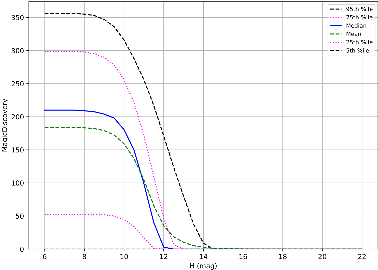
too_combined_no_gw_s10.0_v3.4_10yrs: OCC_r20 6 detections in 60 nights detection loss
