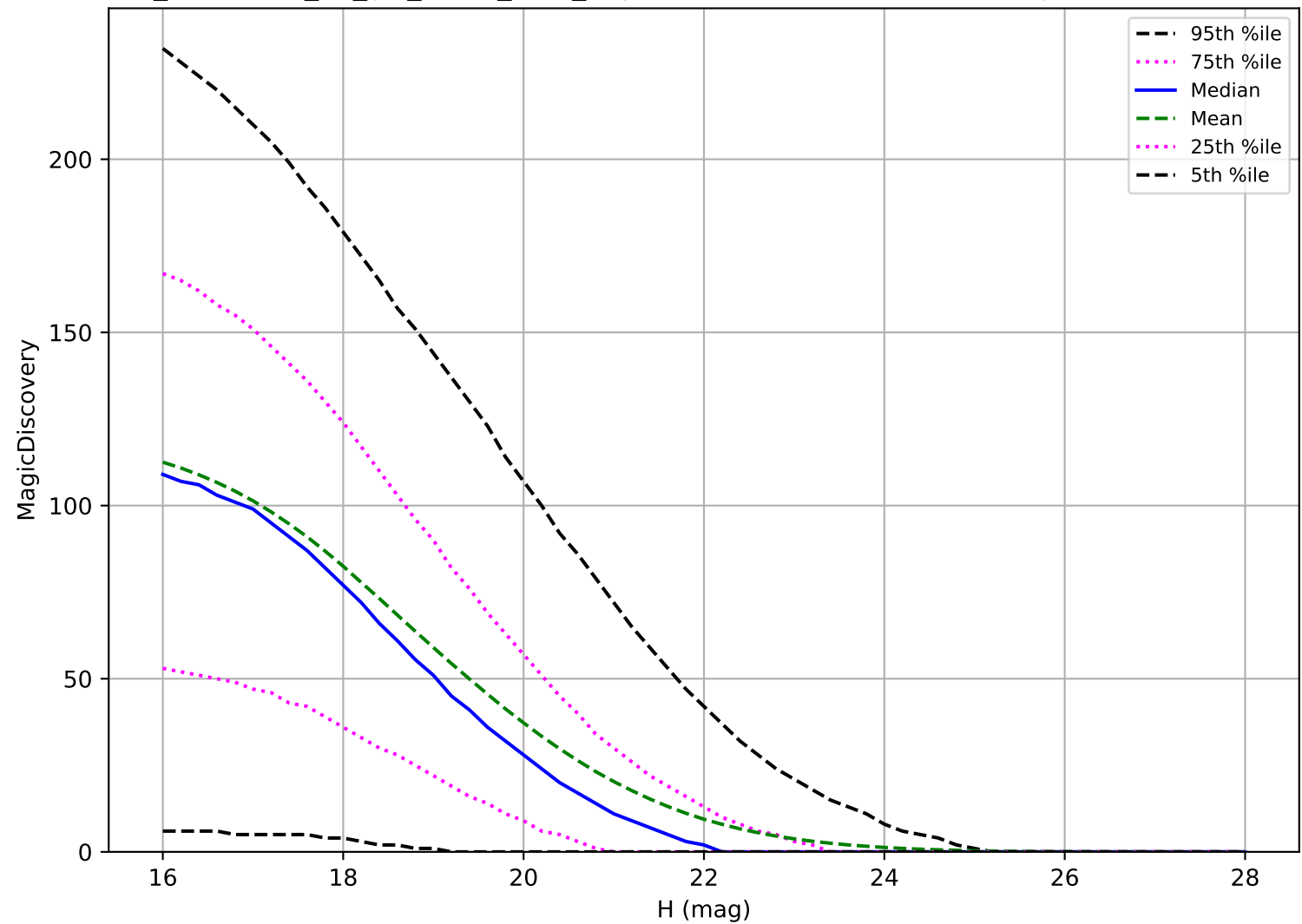
too_combined_no_gw_s10.0_v3.4_10yrs: NEO 6 detections in 60 nights detection loss
