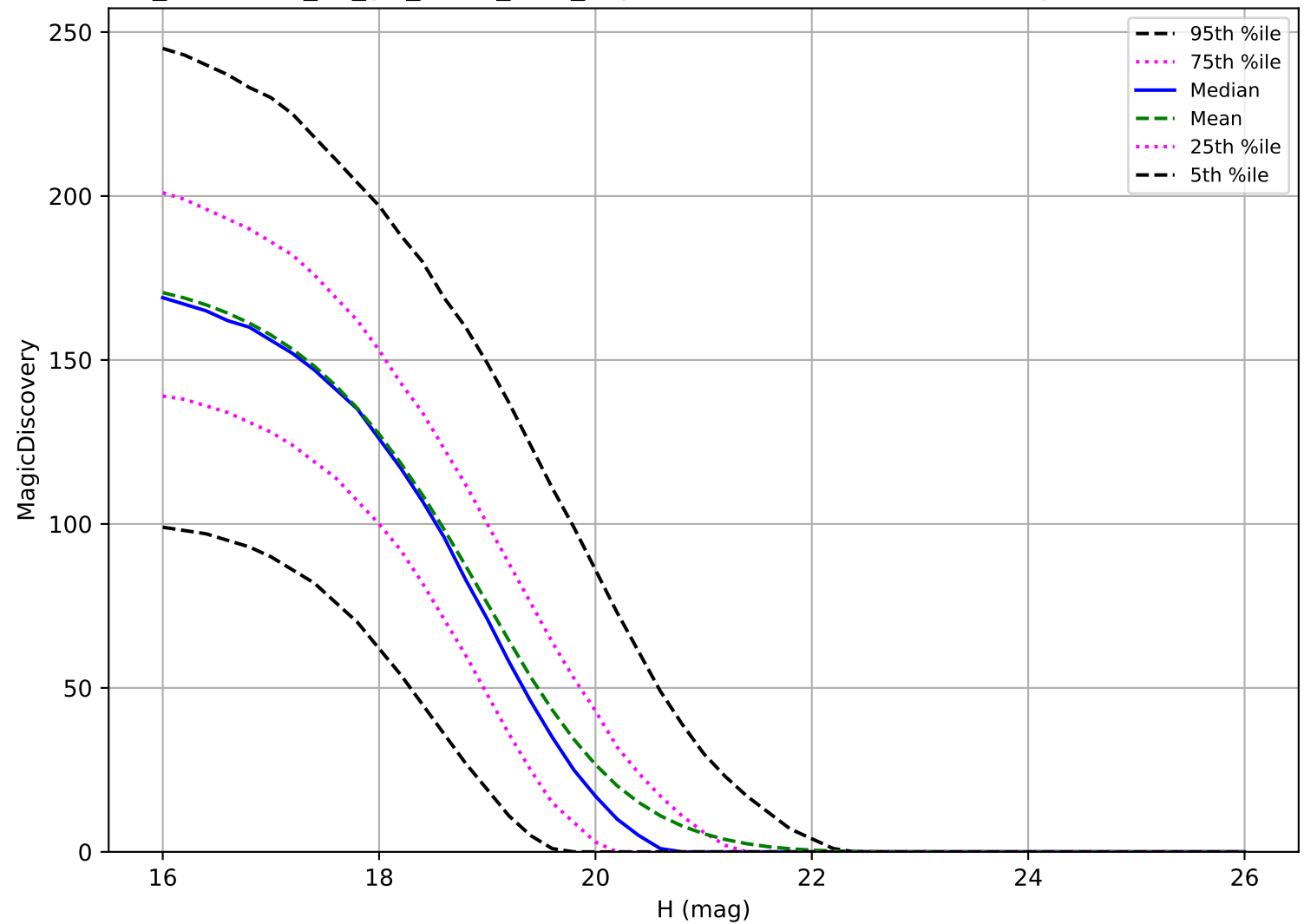
too_combined_no_gw_s10.0_v3.4_10yrs: MBA 6 detections in 60 nights detection loss
