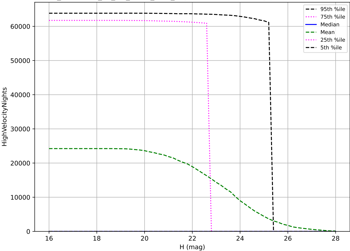
too_combined_no_gw_s10.0_v3.4_10yrs: PHA High velocity pair detection loss
