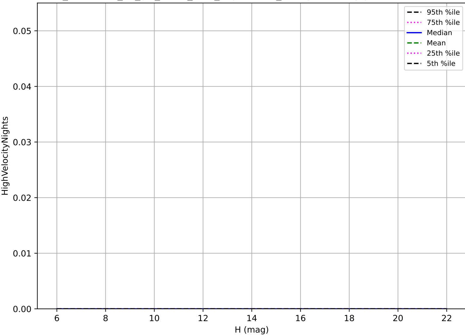
too_combined_no_gw_s10.0_v3.4_10yrs: OCC_r5 High velocity pair detection loss
