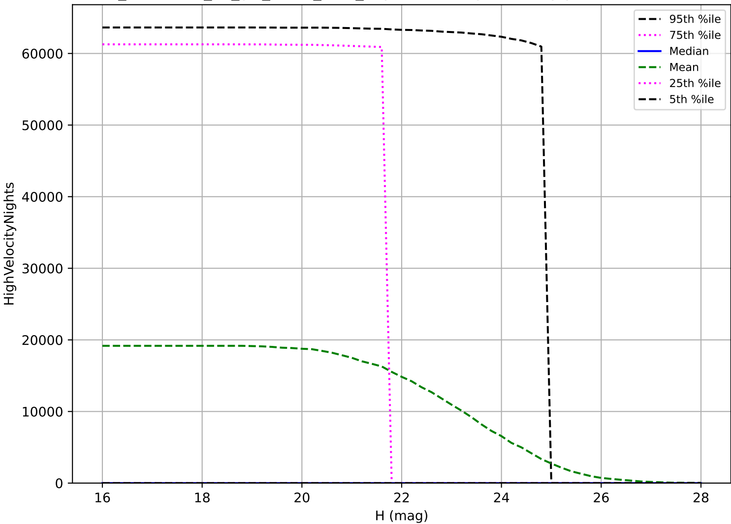
too_combined_no_gw_s10.0_v3.4_10yrs: NEO High velocity pair detection loss
