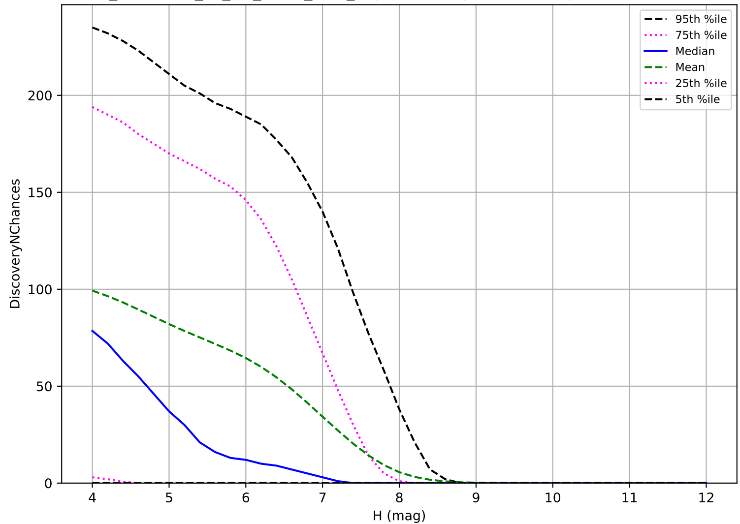
too_combined_no_gw_s10.0_v3.4_10yrs: TNO 3 pairs in 15 nights detection loss
