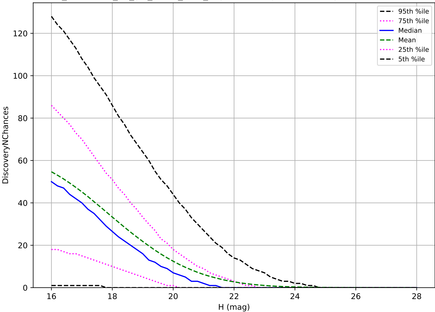
too_combined_no_gw_s10.0_v3.4_10yrs: PHA 3 pairs in 15 nights detection loss
