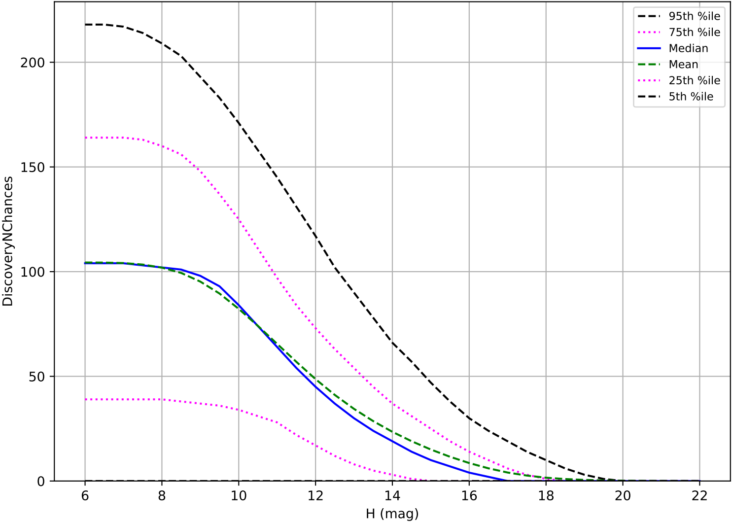
too_combined_no_gw_s10.0_v3.4_10yrs: OCC_r5 3 pairs in 15 nights detection loss
