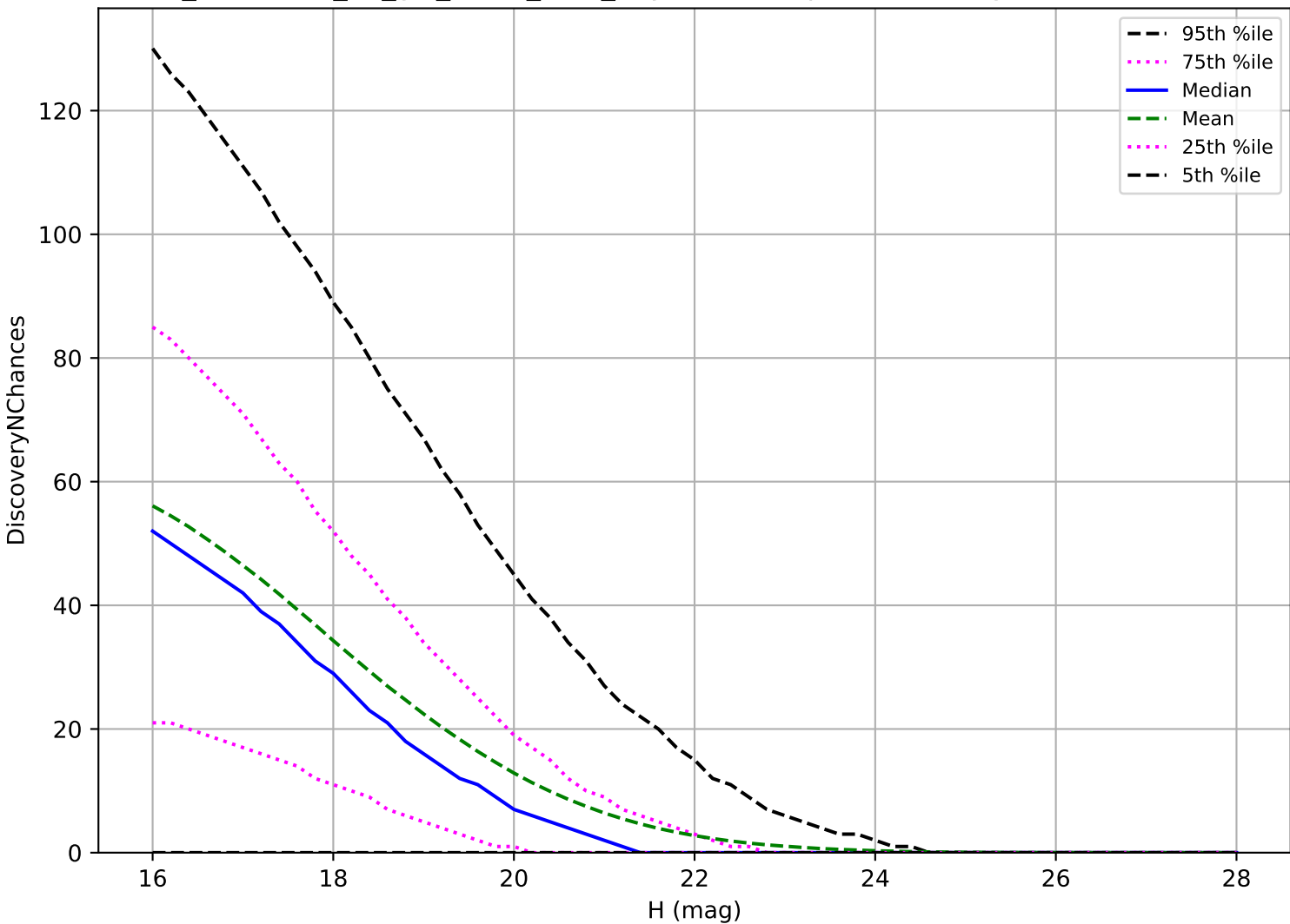
too_combined_no_gw_s10.0_v3.4_10yrs: NEO 3 pairs in 15 nights detection loss
