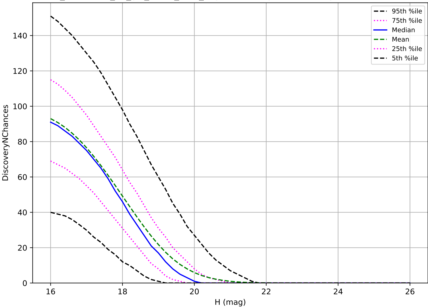
too_combined_no_gw_s10.0_v3.4_10yrs: MBA 3 pairs in 15 nights detection loss
