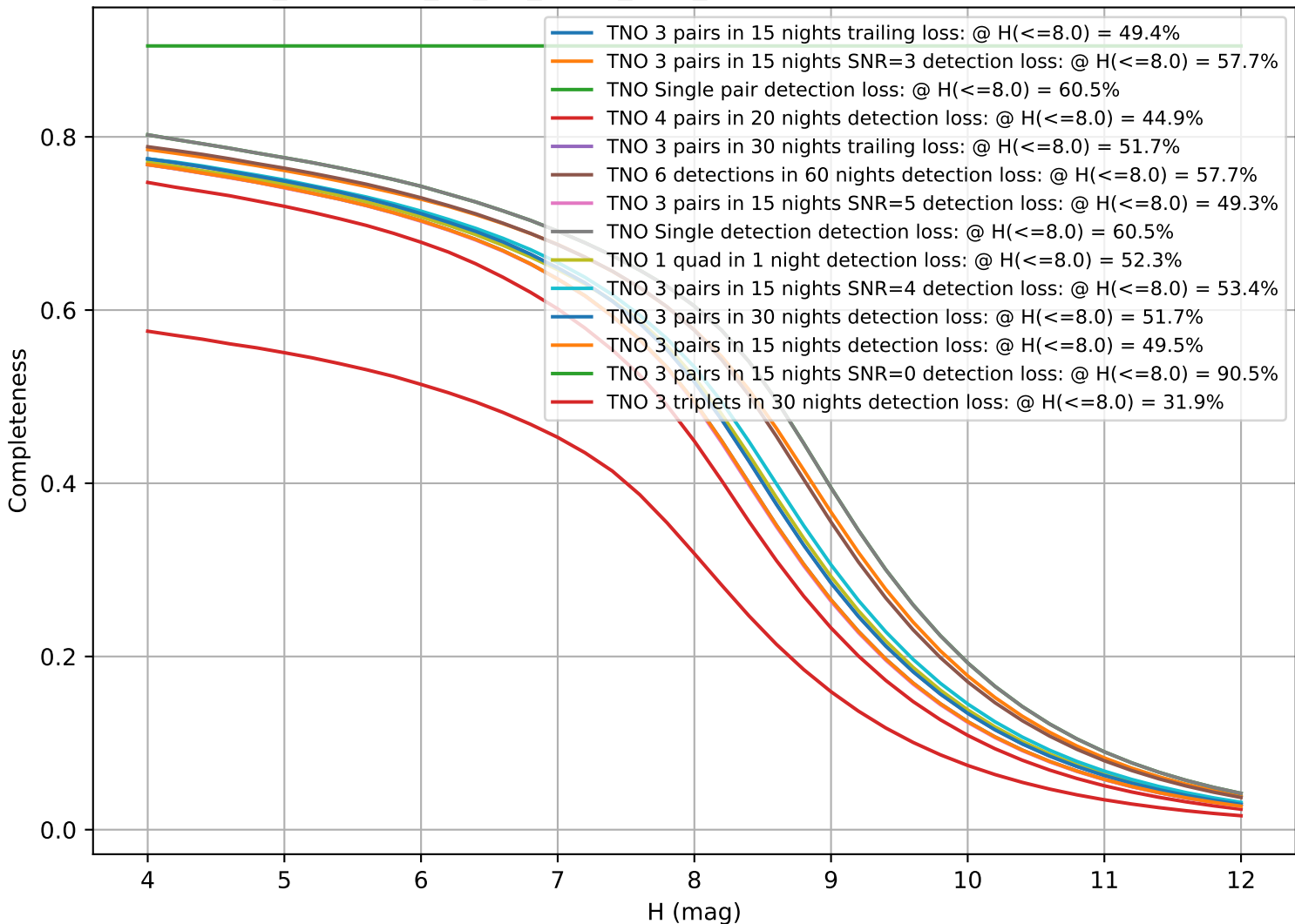
too_combined_no_gw_s10.0_v3.4_10yrs: CumulativeCompleteness
