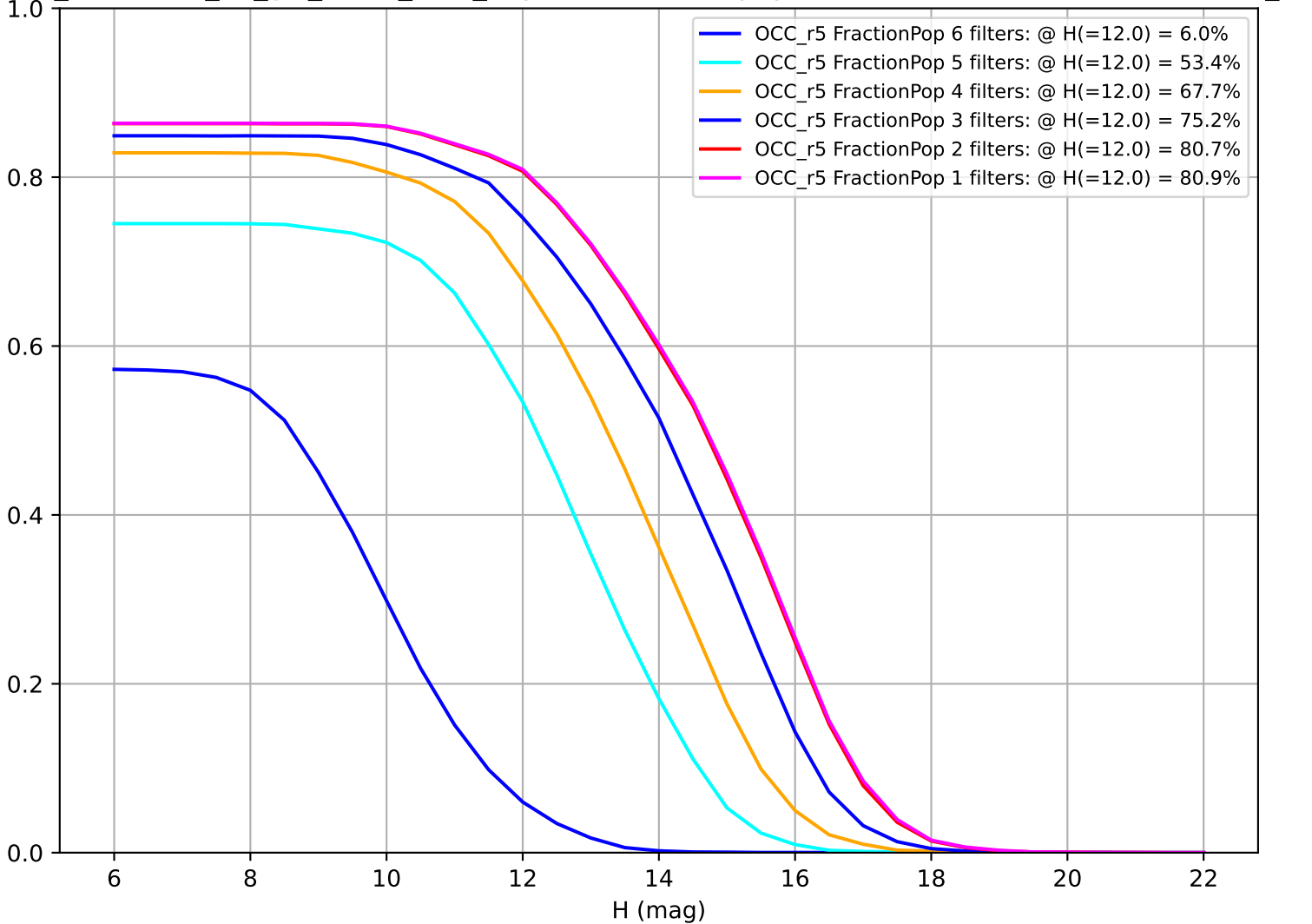
too_combined_no_gw_s10.0_v3.4_10yrs: Fraction of population with colors in X filters OCC_r5
