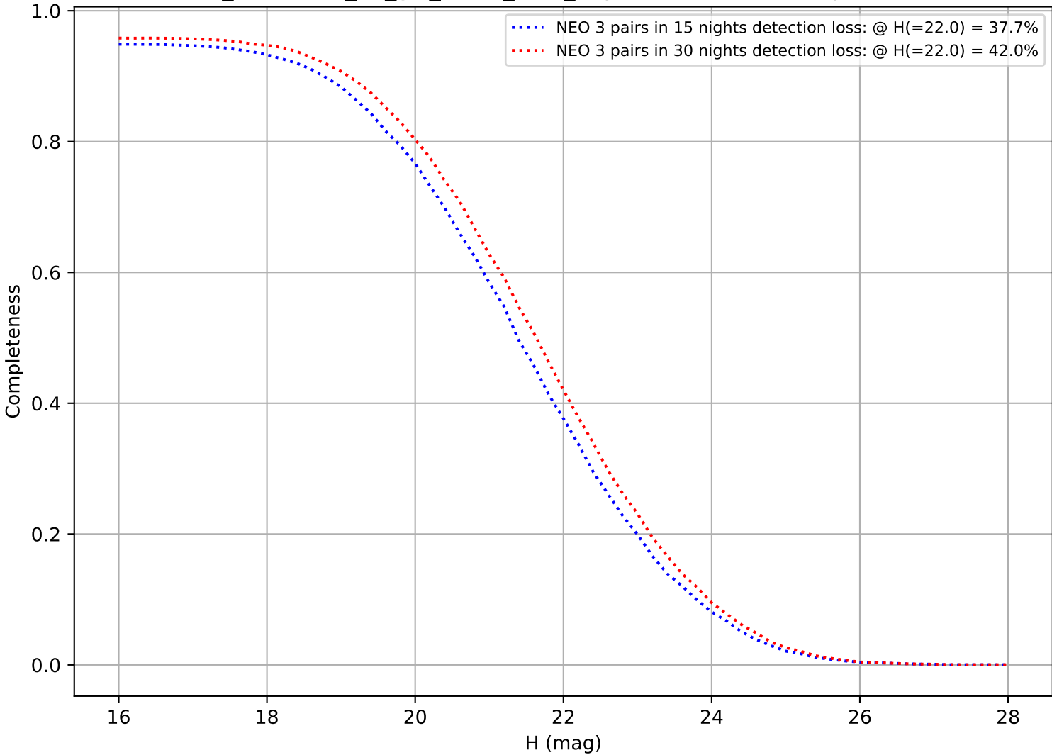
too_combined_no_gw_s10.0_v3.4_10yrs: DifferentialCompleteness
