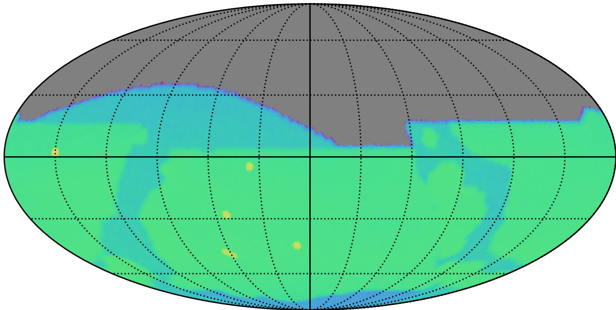
too_combined_no_gw_s10.0_v3.4_10yrs r: SurfaceBrightLimit
