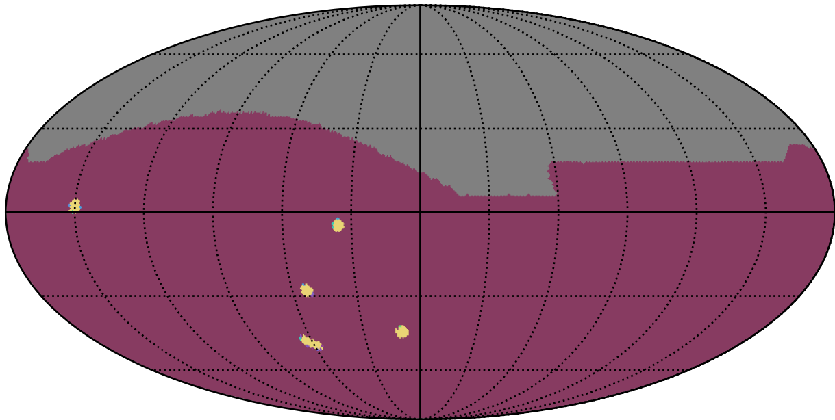
too_combined_no_gw_s10.0_v3.4_10yrs : NumberOfQuickRevisits
