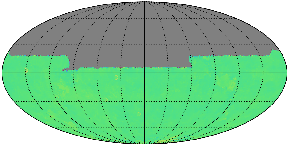
too_combined_no_gw_s10.0_v3.4_10yrs y: Kuiper rotTelPos
