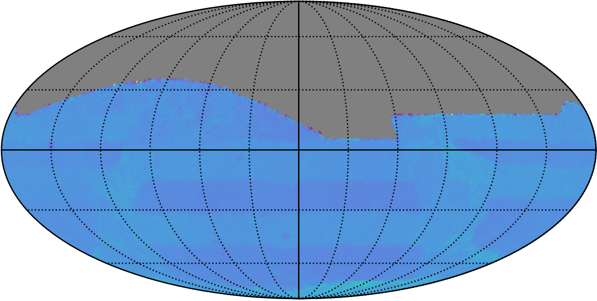
too_combined_no_gw_s10.0_v3.4_10yrs All sky: Normalized Proper Motion Uncert @ 20.5
