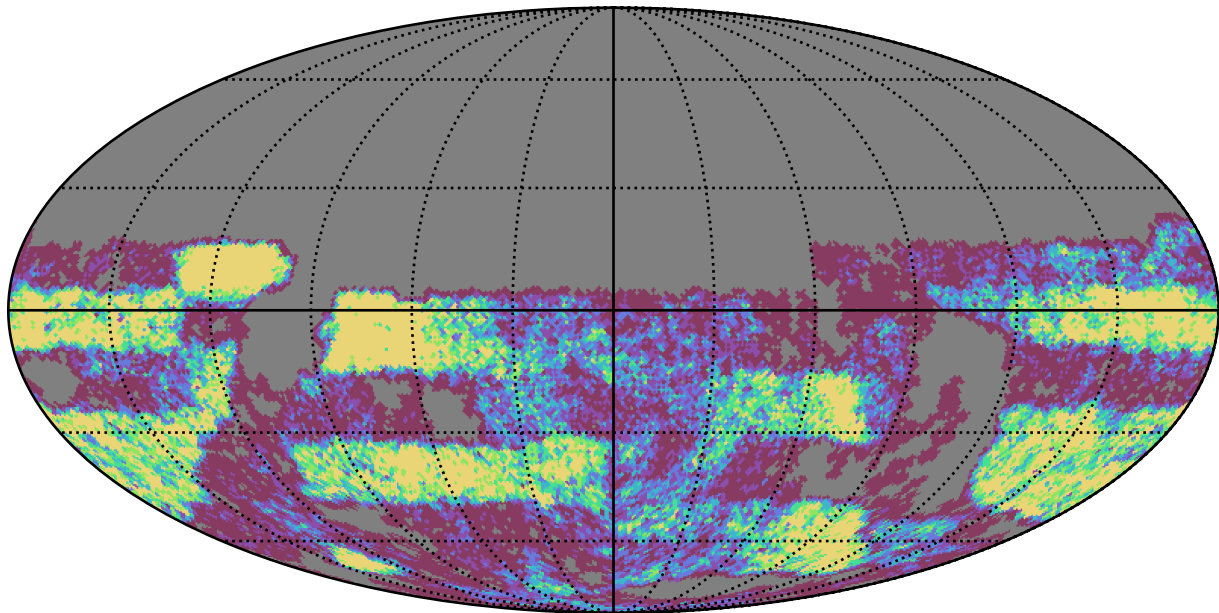
too_combined_no_gw_s10.0_v3.4_10yrs Yr 3-4 u band: NVisits
