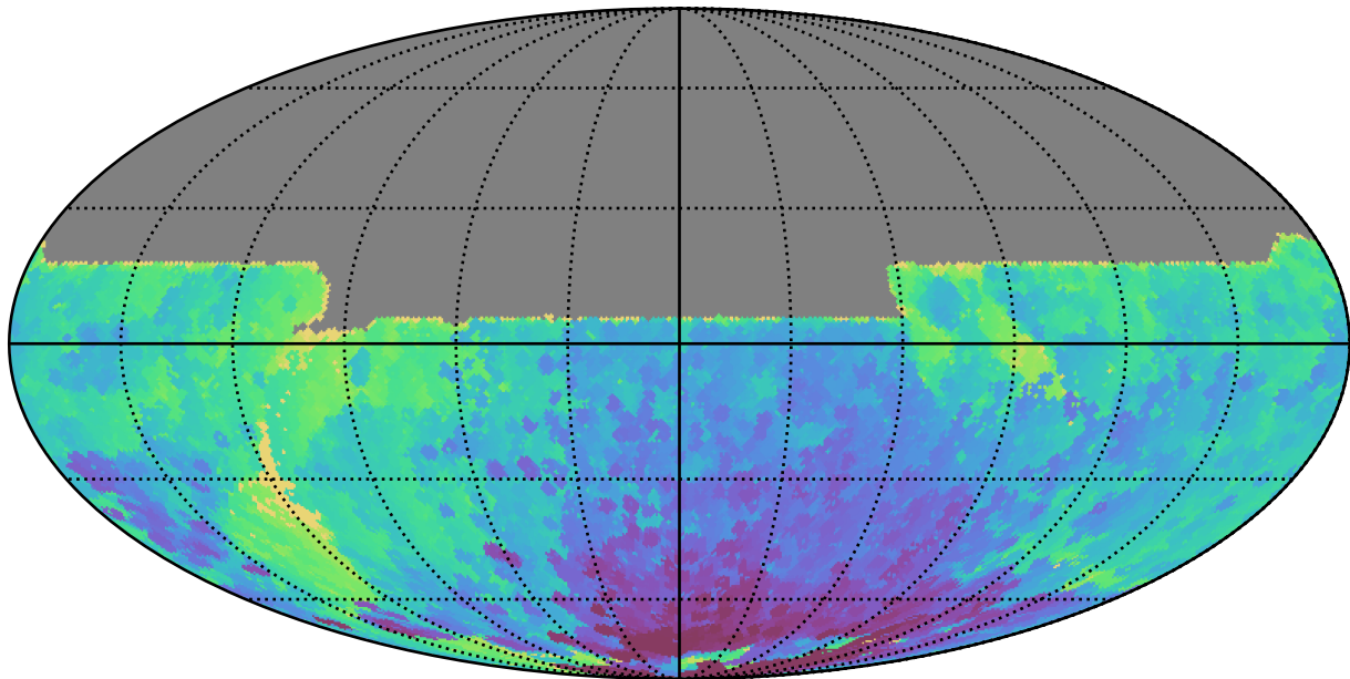
too_combined_no_gw_s10.0_v3.4_10yrs All sky y band: Min HA
