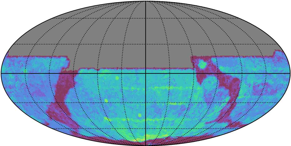
too_combined_no_gw_s10.0_v3.4_10yrs All sky y band: Median Season Length
