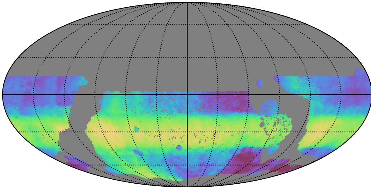
too_combined_no_gw_s10.0_v3.4_10yrs WFD r band: Median HA
