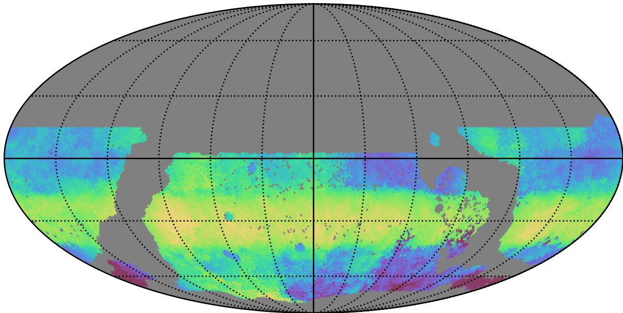
too_combined_no_gw_s10.0_v3.4_10yrs WFD g band: Median HA
